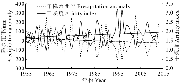
图 1 董志塬 1955—2013 年干燥度和降水距平图 Fig.1 The varieties of aridity index and precipitation anomaly in Dongzhi Loess Tableland from 1955 to 2013
