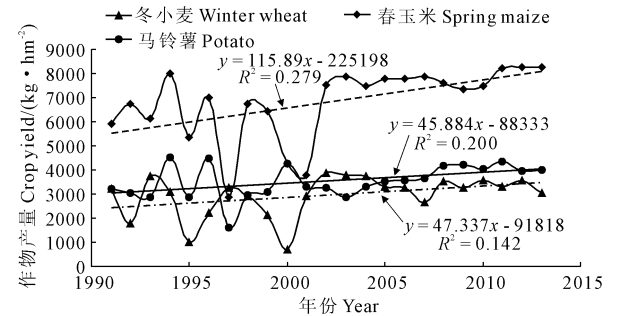
图 2 董志塬 1991—2013 年冬小麦、春玉米和马铃薯单位面积产量图 Fig.2 The yield of winter wheat, spring maize and potato from 1991 to 2013 in Dongzhi Loess Tableland
